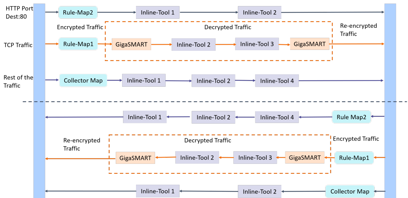
Figure 50 Flexible Inline Decryption Solution
