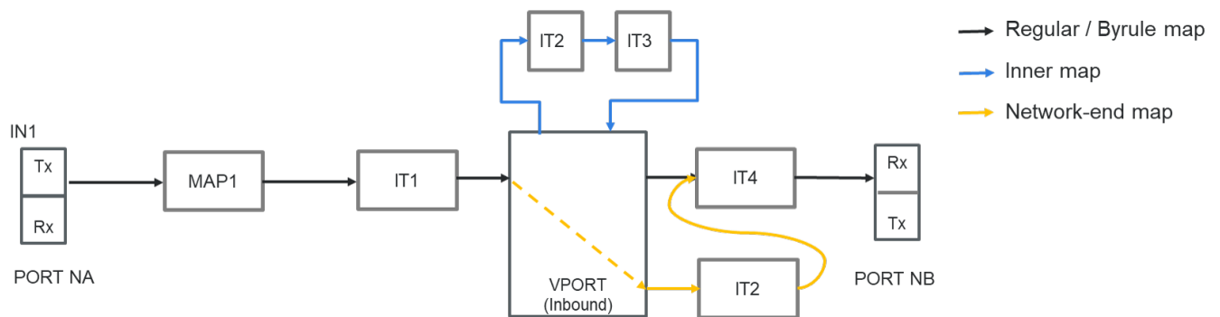
Figure 51 Flexible Inline Decryption Maps
