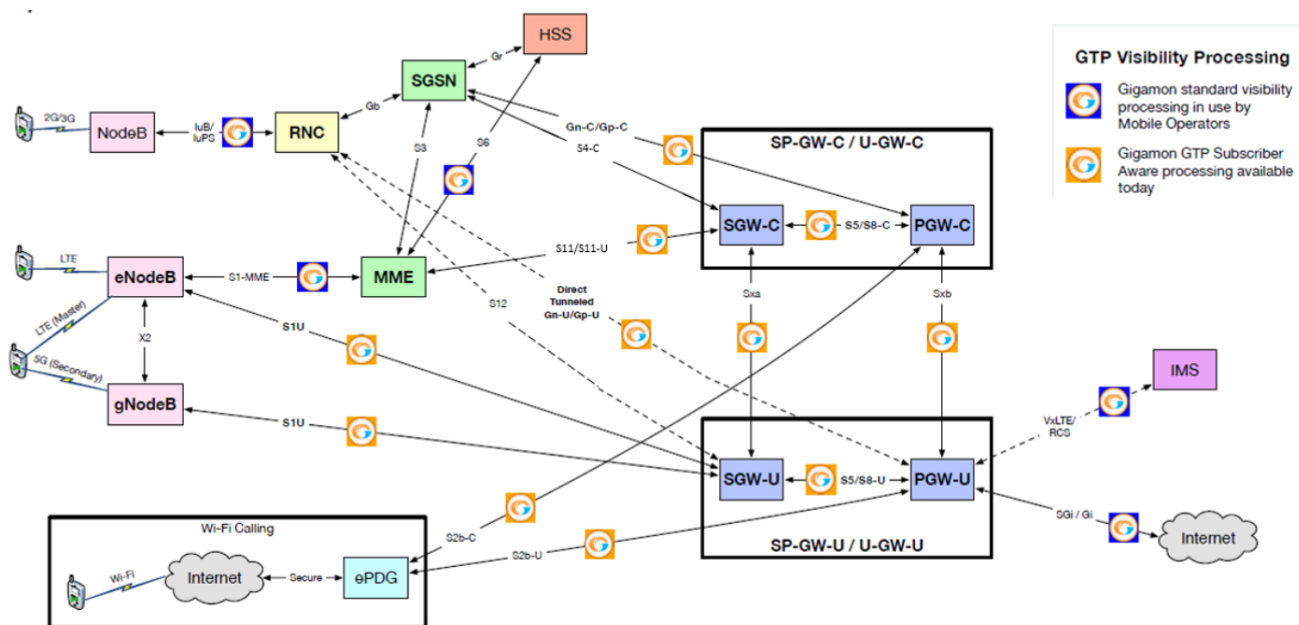
Figure 30 3GPP CUPS Network topology
